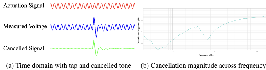
Fig. 1: Cancellation shown with example signal and cancellation across frequency
